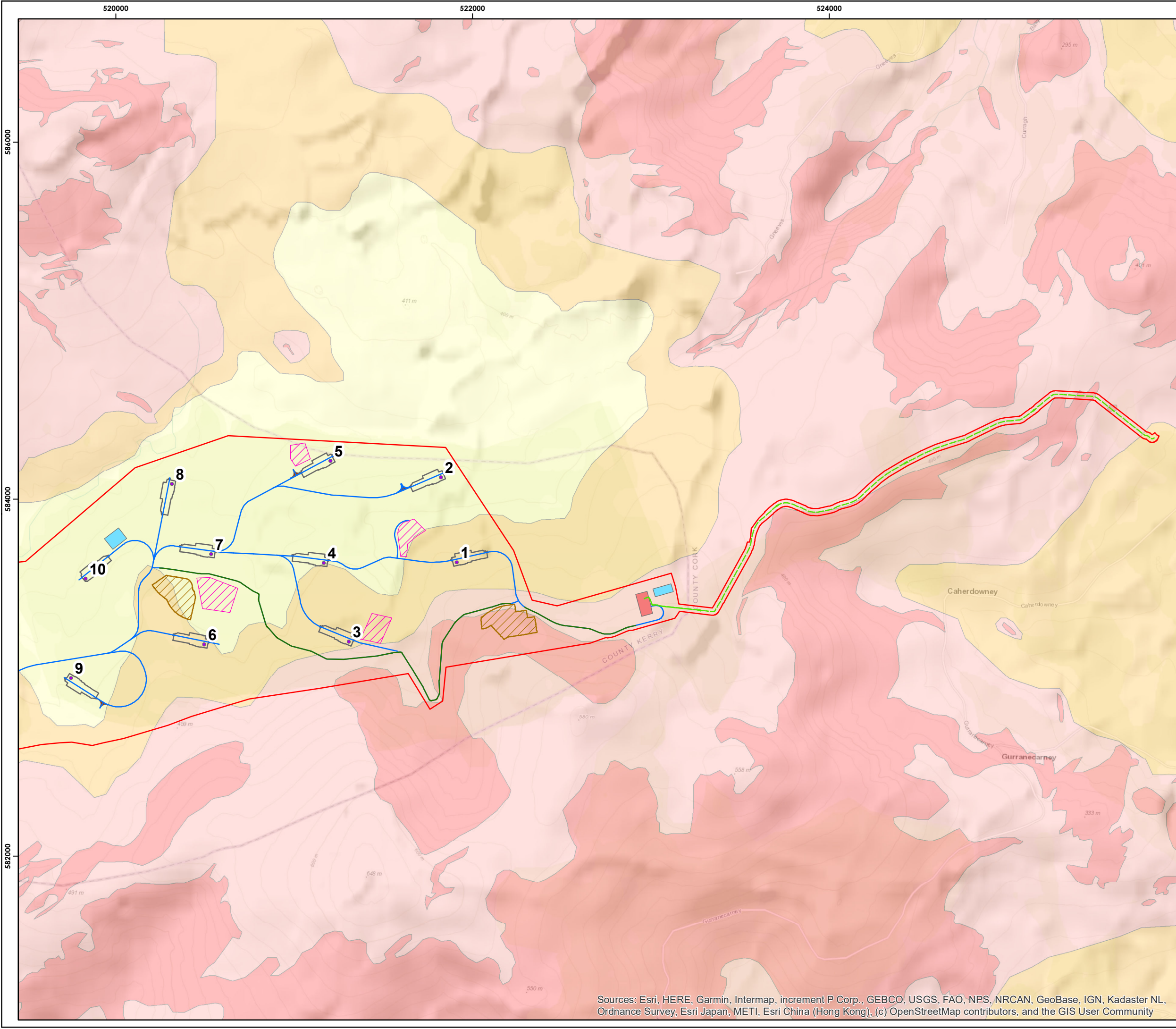
Figure10-7c Groundwater Vulnerability
